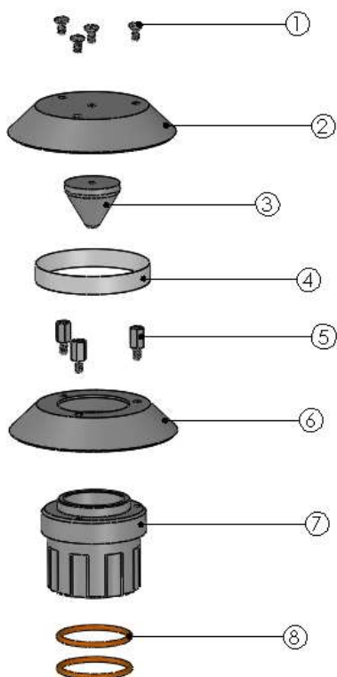
PM 10 Louvered Inlet Assembly
